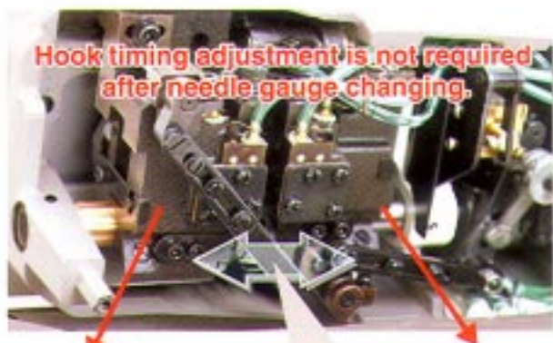
Hook driving shaft saddle (left)
