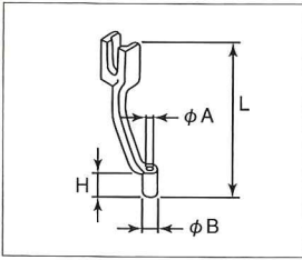
Intermediate presser
