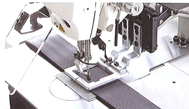
Example application: Reinforcing the stitching of seatbelts *The feeding frame is special order item.
