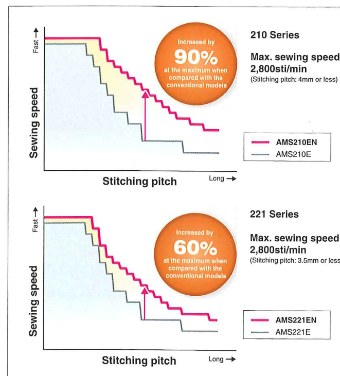
Comparison between stitching pitch and sewing speed
