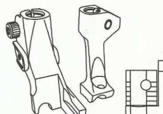
Piping operation to the left of the needle 左坑，繩管用單右趾壓腳
