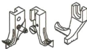
Feeding foot with compensating guide, toe on left side 高低傍位內壓腳，趾在左邊
