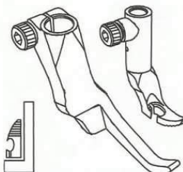
Left cording foot set 左單邊壓腳
