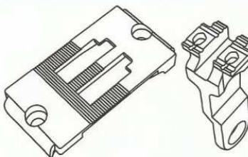
Needle plate & feed dog for 1296 with thread trimmer 1296 剪線用針板/送布牙
