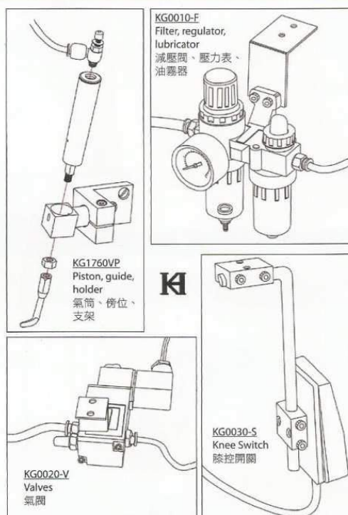
Pneumatic guiding set with F.R.L. unit, knee switch and valves for Juki PLC-1760 重機PLC-1760 氣動傍位連 F.R.L. 聯組、氣閥、膝控開關
