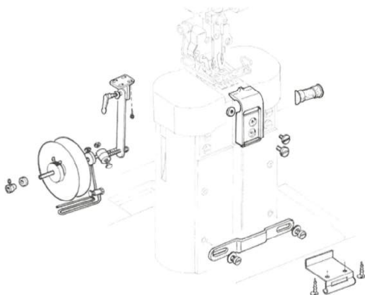
Belt guide completed set for 20mm belt 送縫條套裝 (20mm)
