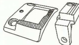
Feed dog wide 牙面寬: 11.4mm Needle plate and feed dog for binding on 205-370 machine, use together with KP205B 205-370用包邊針板/送布牙，需與 KP205B 一同使用
