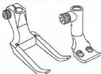
Double needle presser feet set 雙針壓腳
