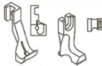
Piping feet 繩管壓腳 From groove to needle hole 針孔至繩坑: 0mm
