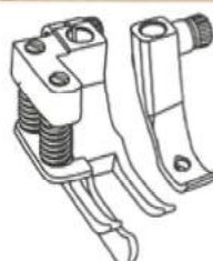
Deeper left compensating guide with balancing spring for EXTREME HEAVY DUTY 左邊彈弓傍位壓腳，超厚物用
