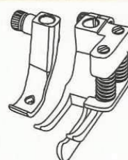
Deeper right compensating guide with balancing spring for EXTREME HEAVY DUTY 右邊彈弓傍位壓腳，超厚物用
