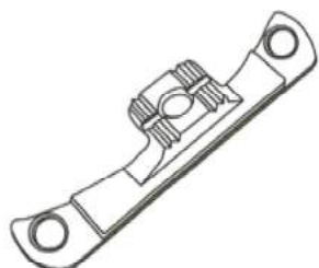
Bigger needle hole: 4.2 x 3.2mm 大針孔送布牙: 4.2 x 3.2mm
