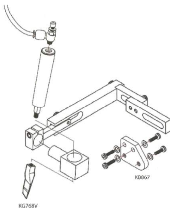
Pneumatic guiding set for 868 868 氣動傍位
