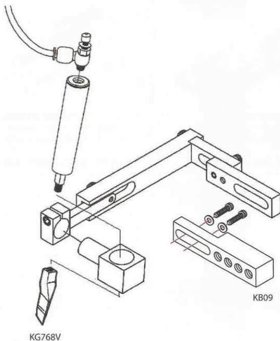
Pneumatic guiding set for most Pfaff post bed machines 百福立柱式縫紉機用氣動傍位
