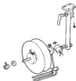
Under table tape roller holder 桌下型細條盤
