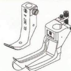
Stronger left compensating guide & wider feeding foot for HEAVY DUTY 特強左邊彈弓傍位壓腳，特闊送料
