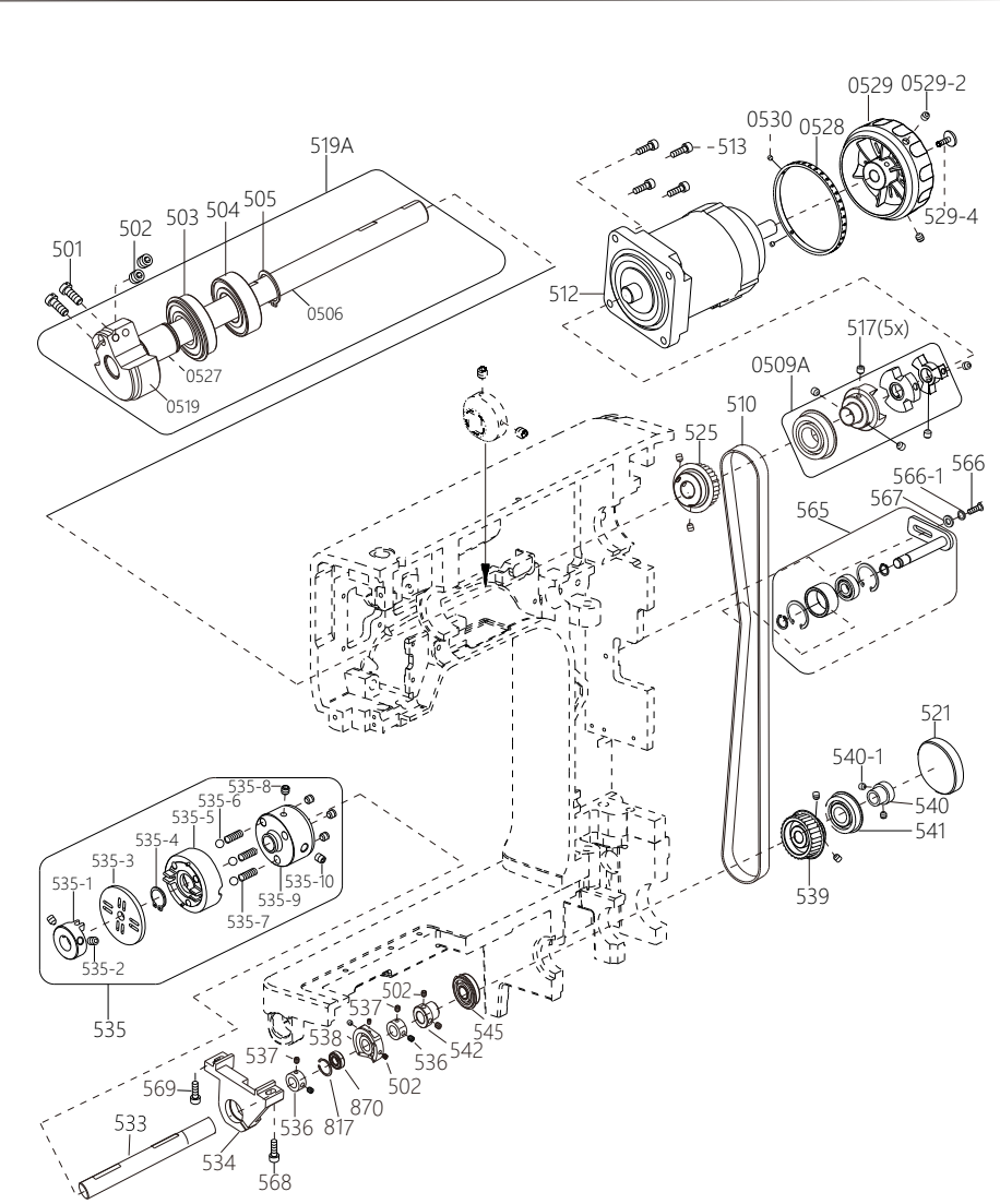
Upper & main shaft transmission mechanism
