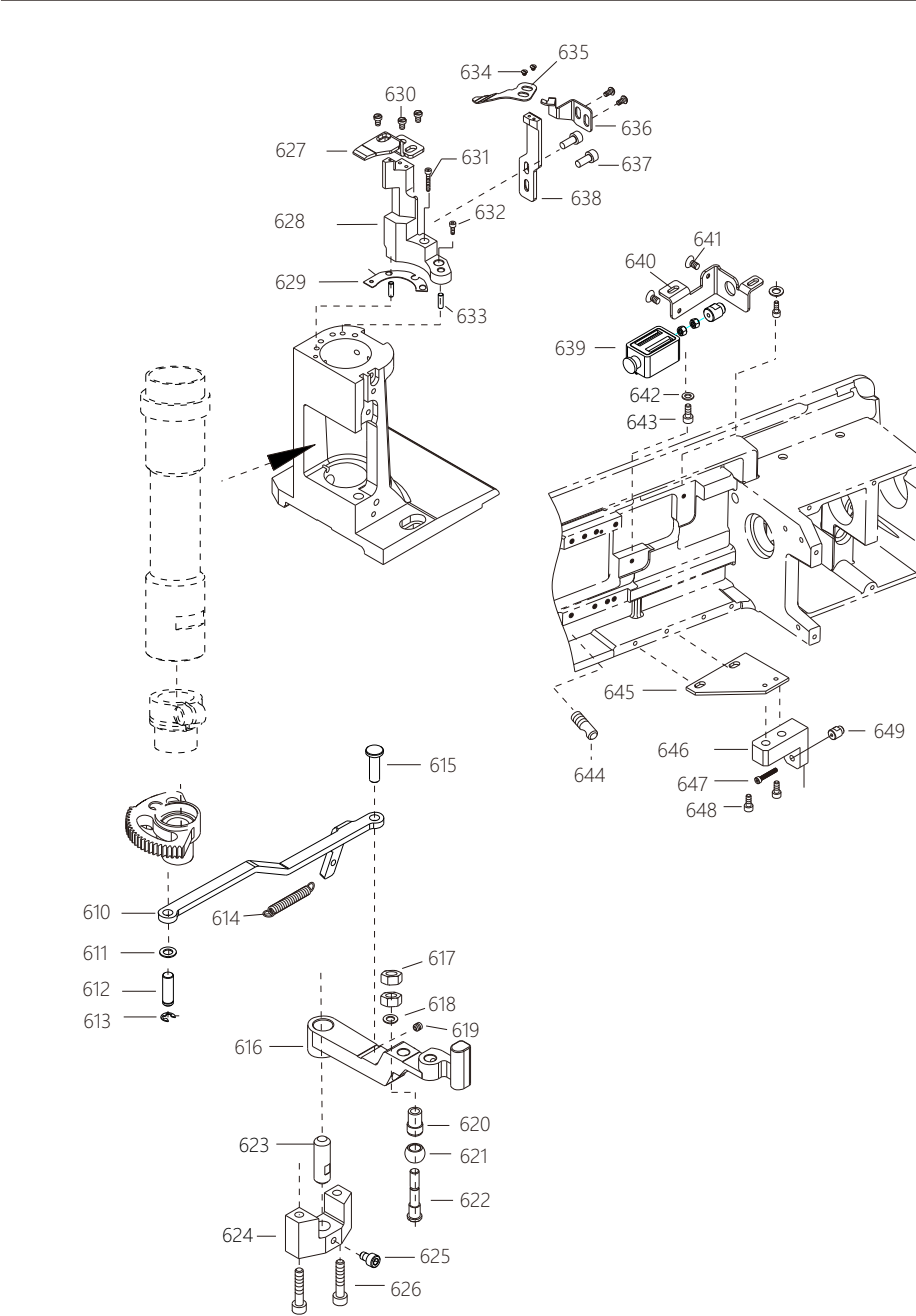
Thread trimming mechanism
