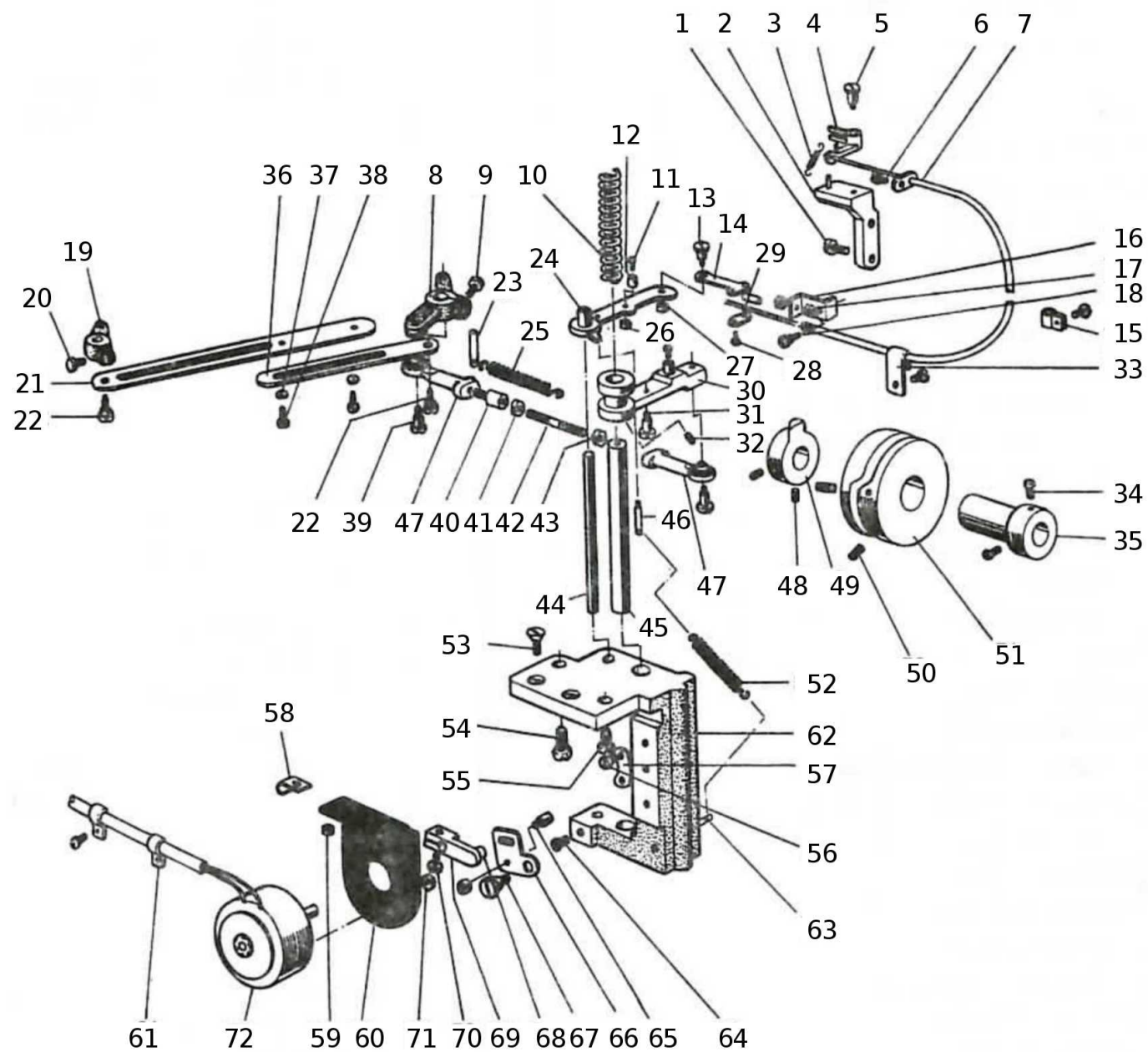
KNIFE MECHANISM
