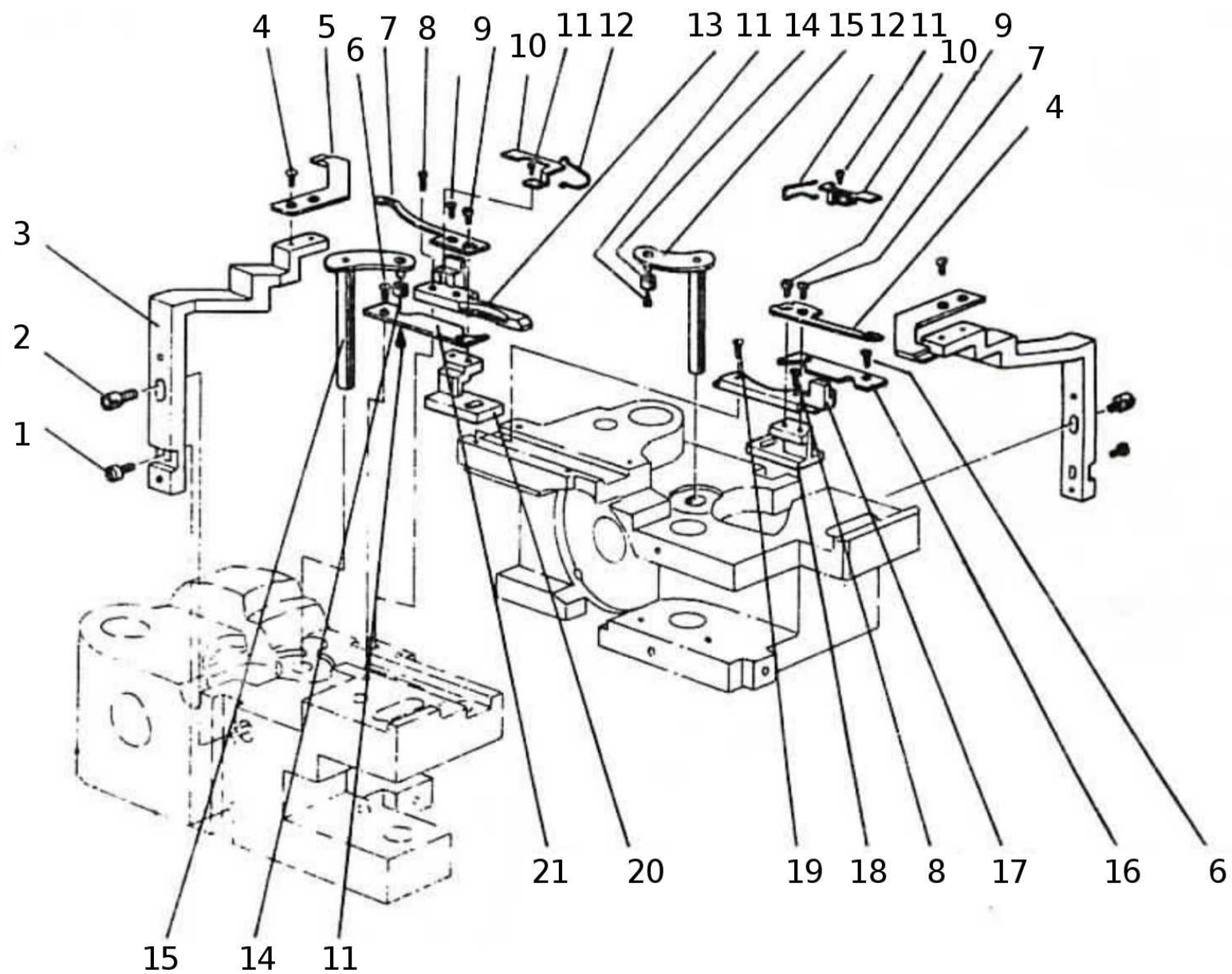
UPPER FEED ROCK SHAFT MECHANISM
