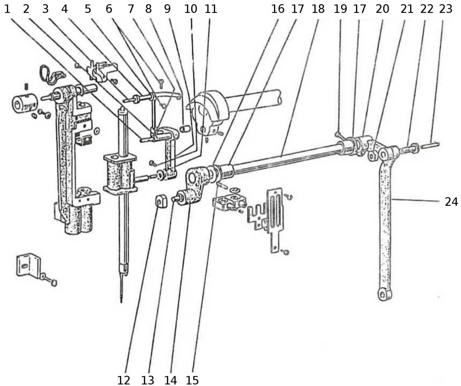
NEEDLE BAR ROCKING MOTION MECHANISM
