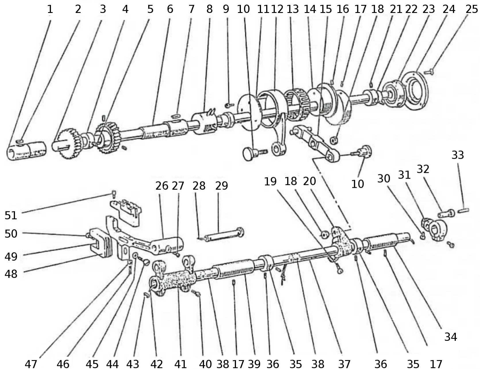
LOWER SHAFT & FEED ROCK SHAFT MECHANISM
