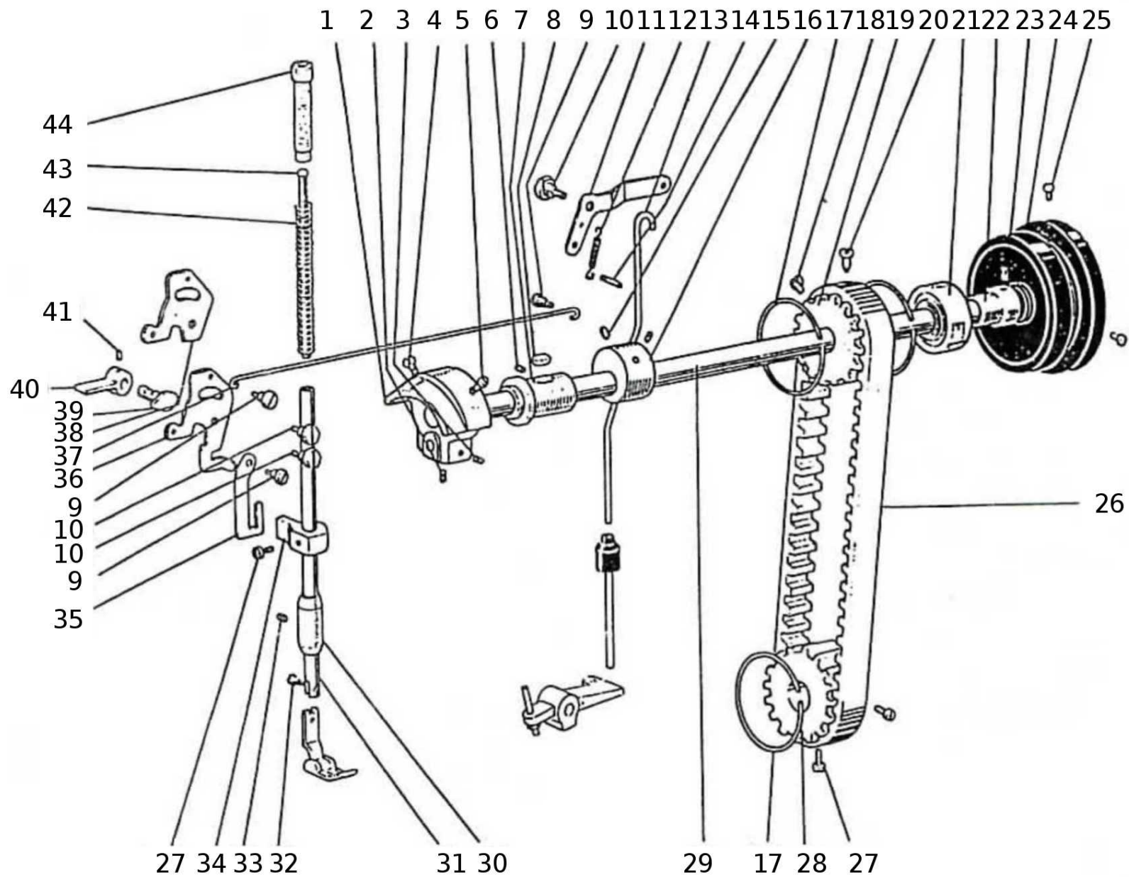
ARM SHAFT MECHANISM
