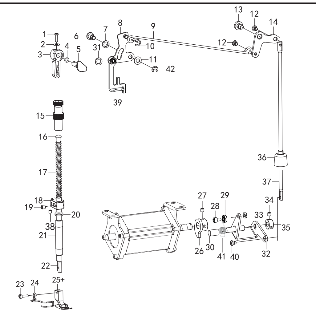
3.压脚装置/Presser foot mechanism
