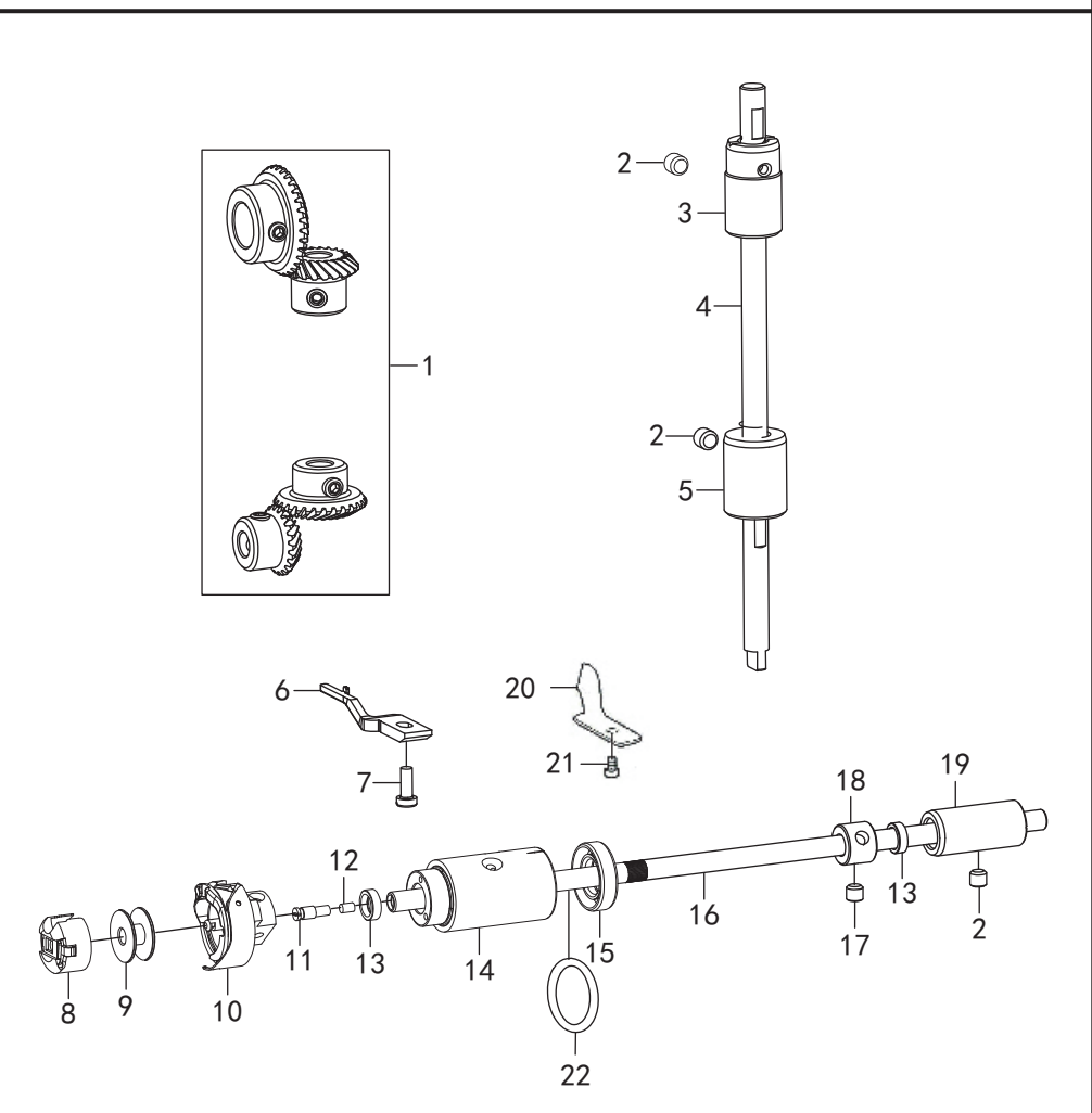
5.旋梭装置/ Hook components
