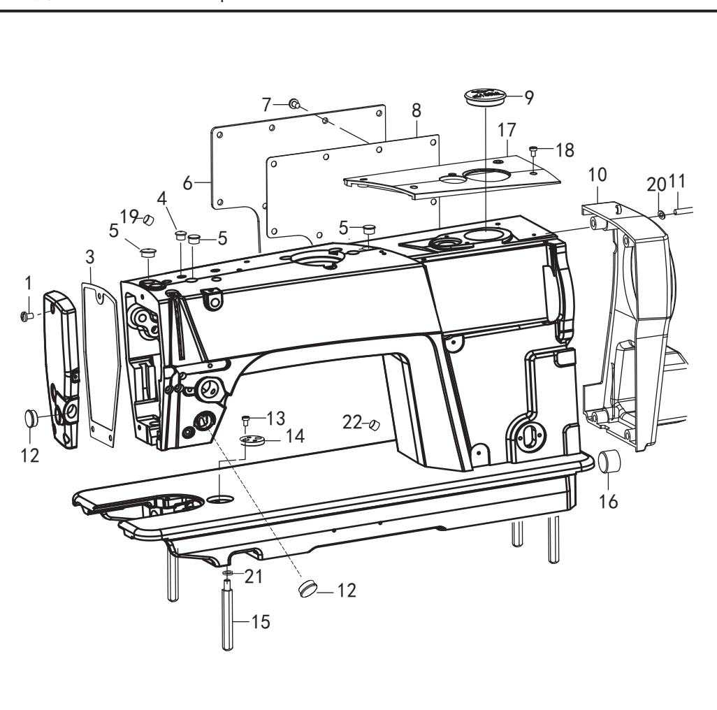
1. 机壳部件 /Arm bed components
