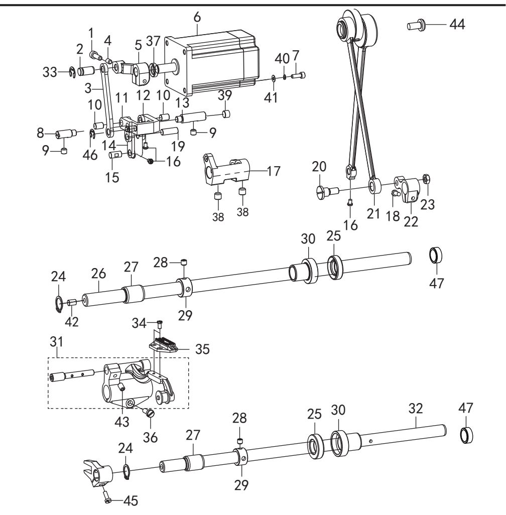
4.送料装置/Feed mechanism components
