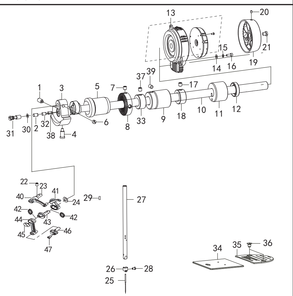
2.上轴装置/Shaft mechanism
