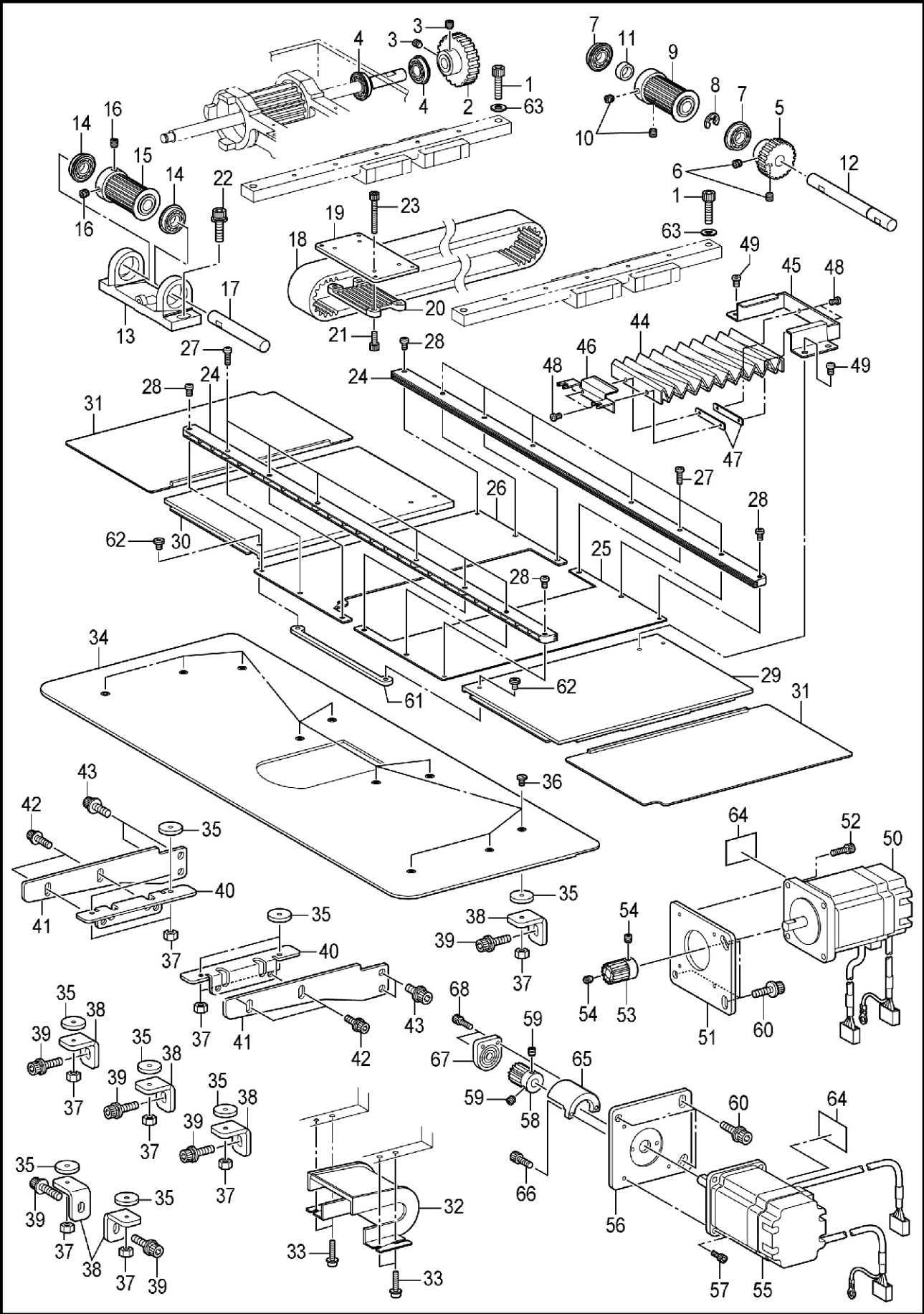
C2. 送料装置 / Feed mechanism
