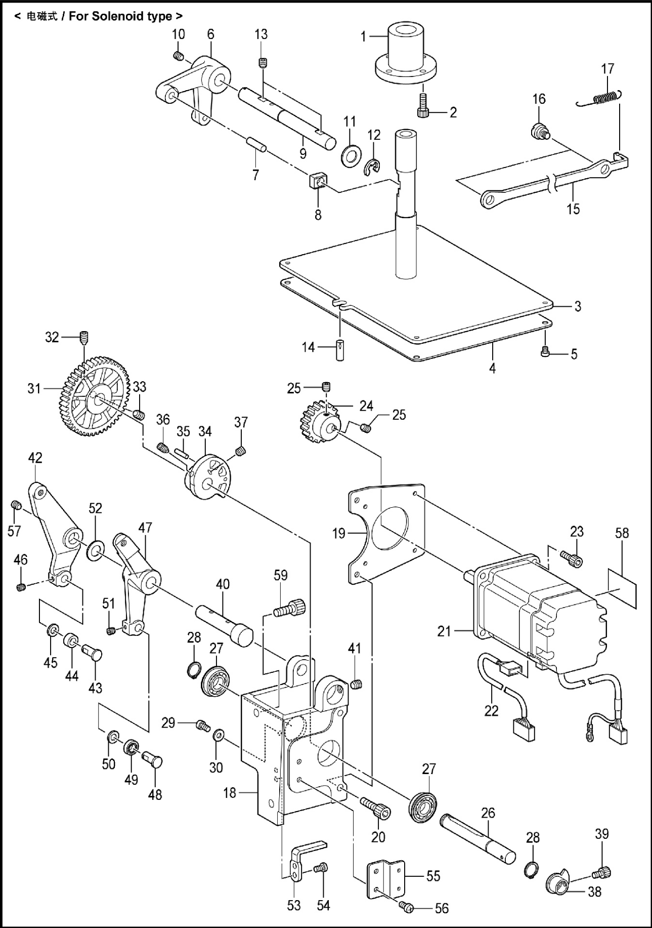
D2 . 抬压装置 / Work clamp lifter mechanism
