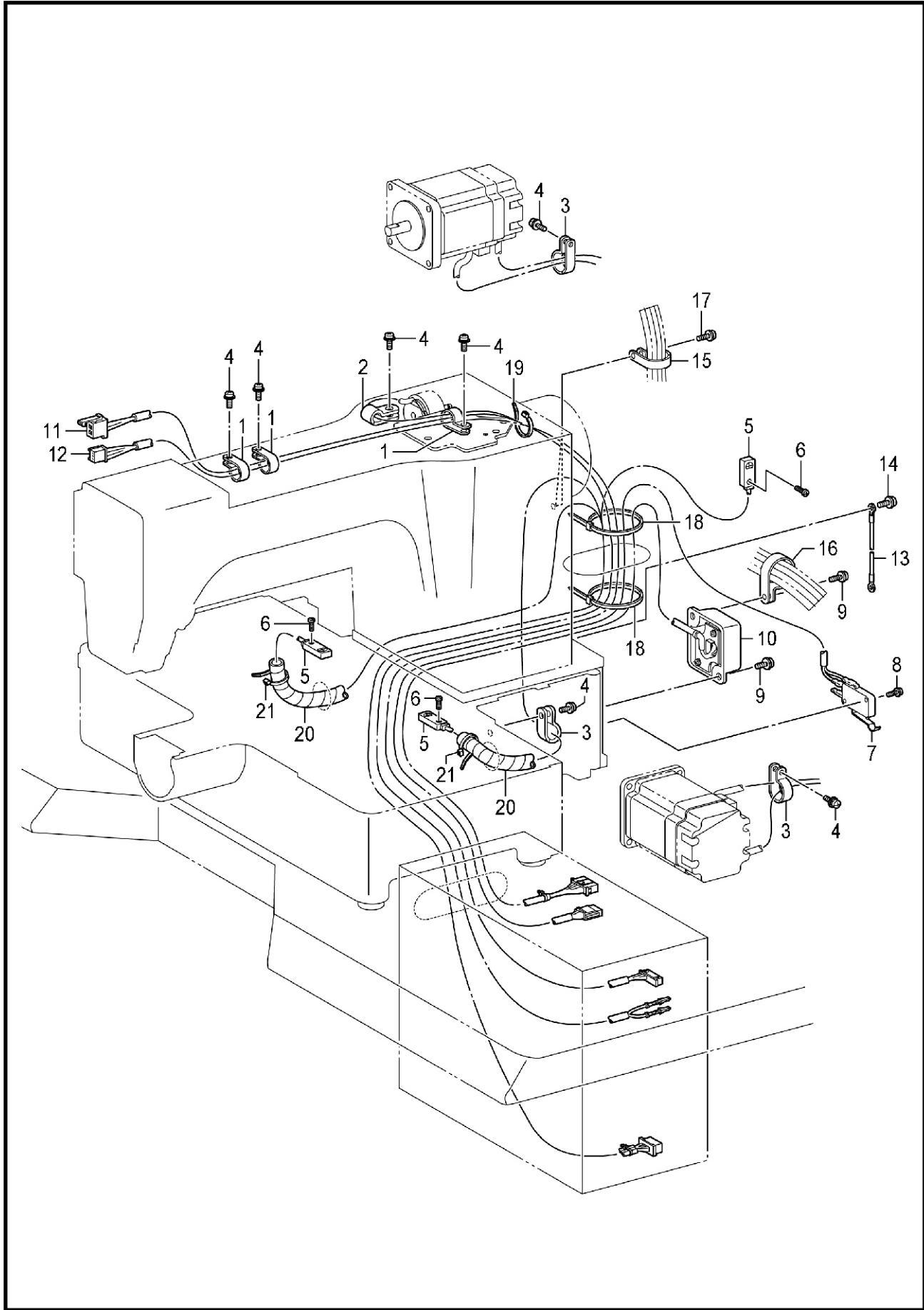
Q . 电气部品装置 / Power supply equipment mechanism
