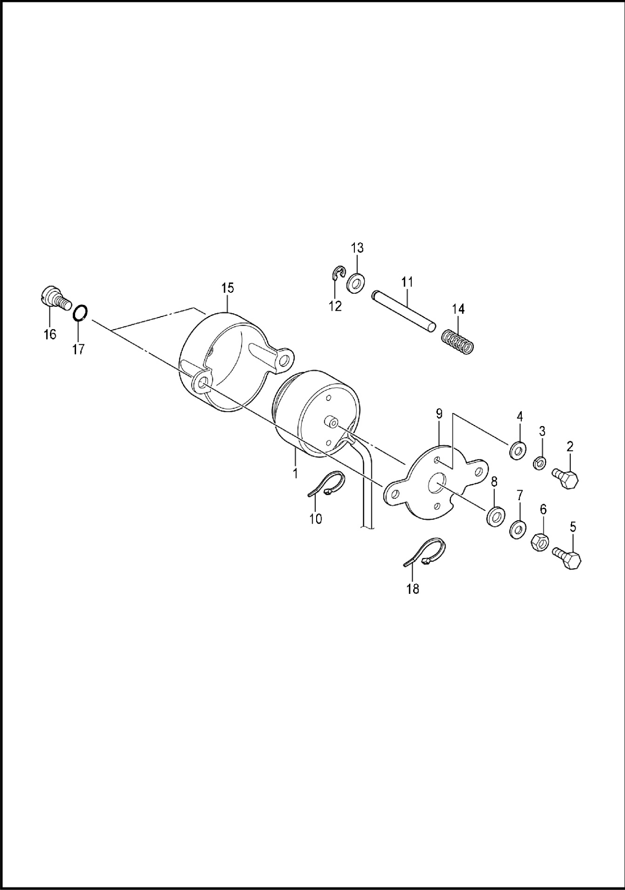
L . 松线装置 / Tension release mechanism
