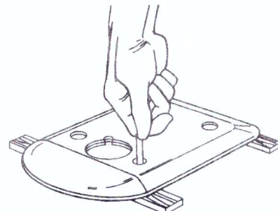
Figure 34. Removing a Worn Plate Roller Shell
