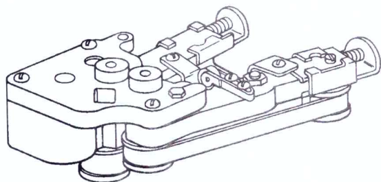
Figure 30. Lower Gear Bracket Assembly (Assembled View)
