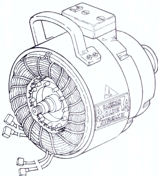
Figure 21. Single-Phase Motor Assembly (Assembled View)
