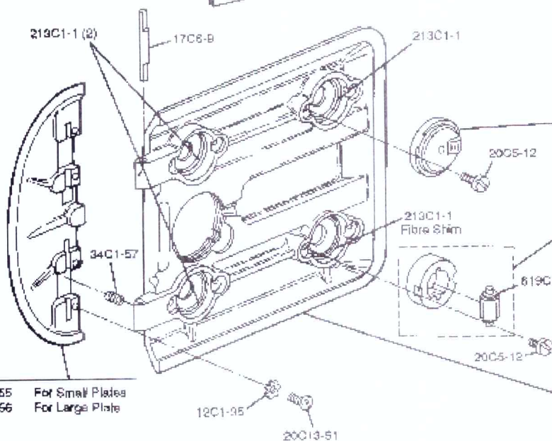
Figure 33. Standard and Baseplate Assembly (Exploded View)
