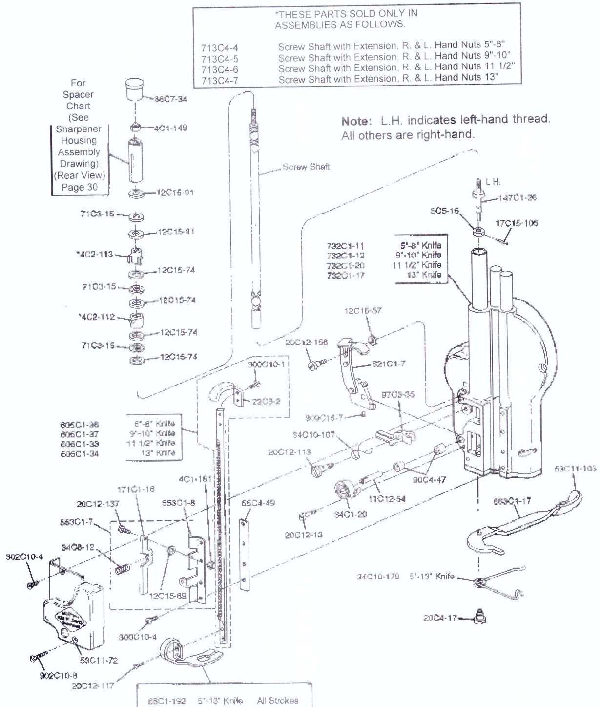
Figure 27. Sharpener Housing Assembly (Exploded, Front View)
