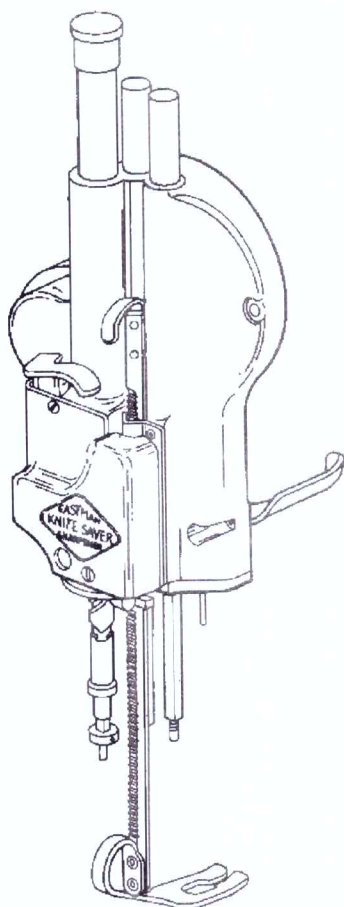
Figure 26. Sharpener Housing Assembly (Assembled, Front View)
