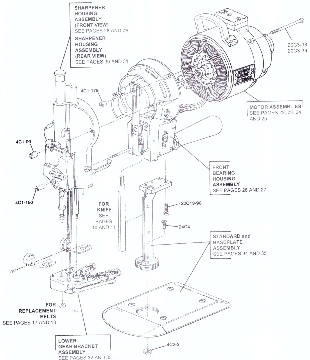
Figure 20. Standard and Baseplate Assembly (Exploded View)
