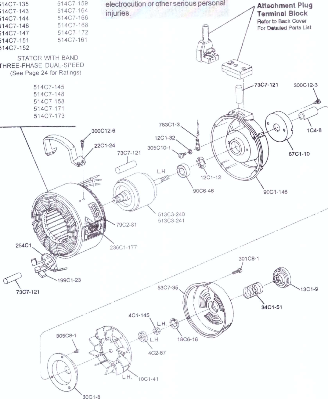
Figure 24. Three-Phase Motor Assembly (Exploded View)
