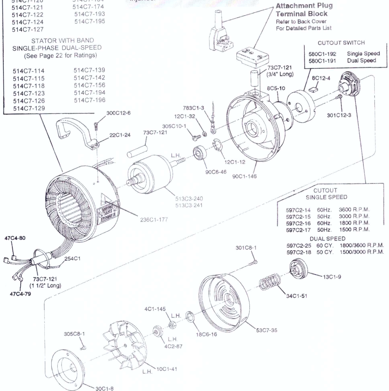
Figure 22. Single/Dual-Phase Motor Assembly (Exploded View)
