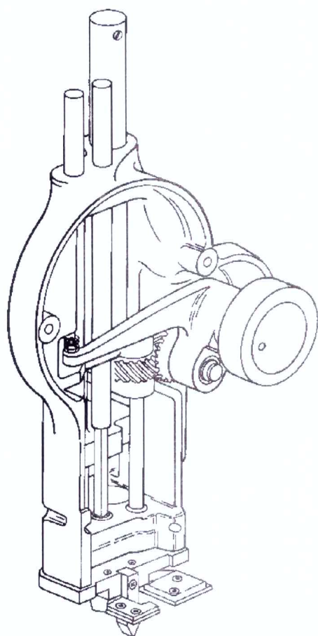
Figure 28. Sharpener Housing Assembly (Assembled, Rear View)
