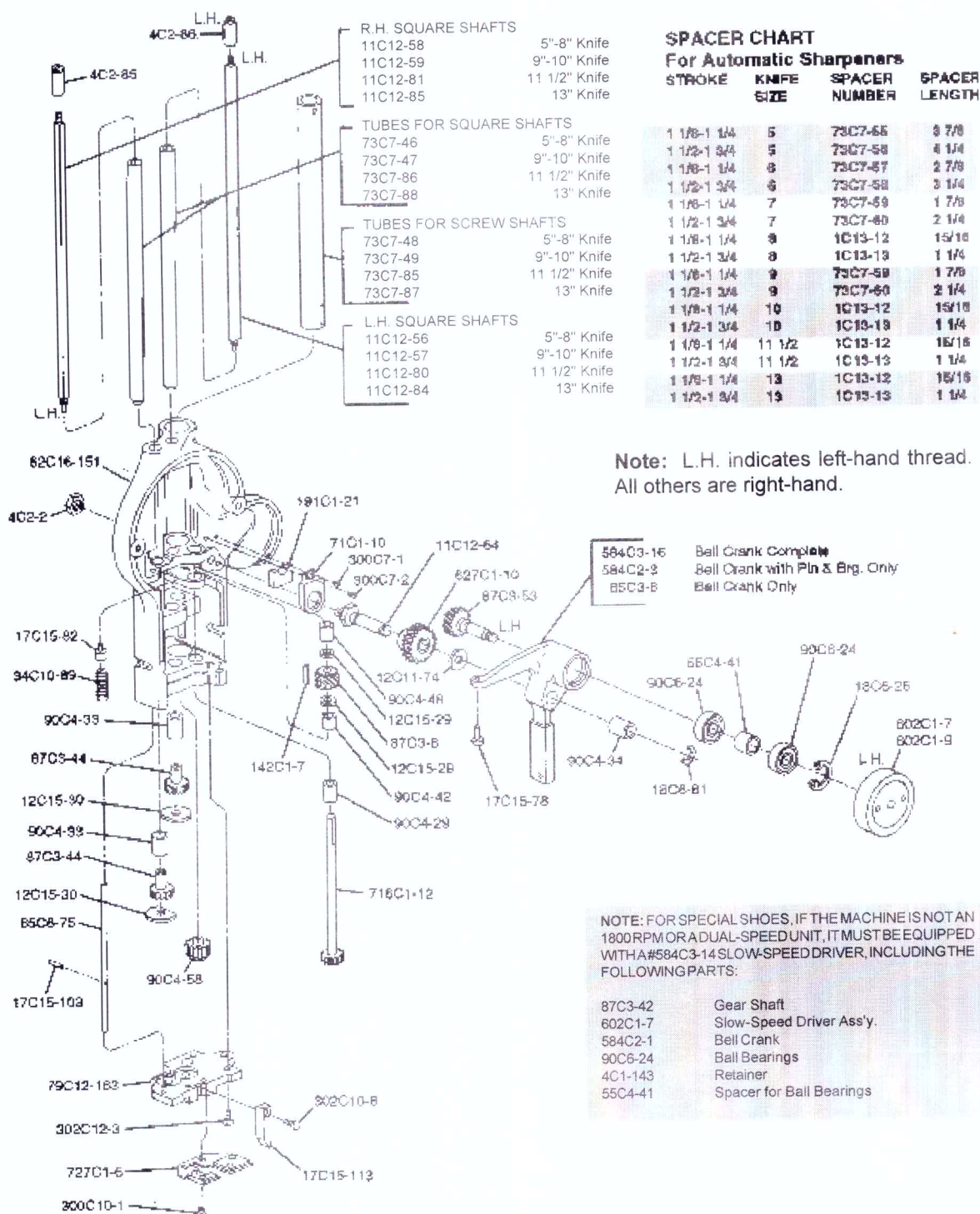
Figure 29. Sharpener Housing Assembly (Exploded, Rear View)
