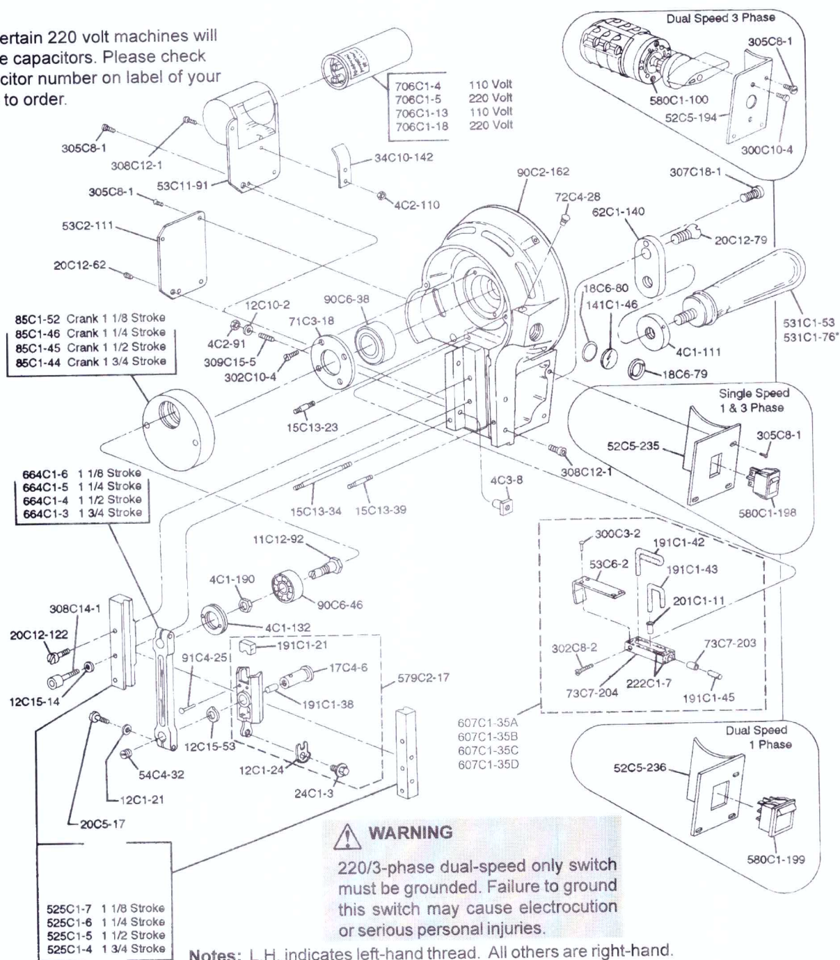
Figure 25. Front Bearing Housing with Oiler Assembly (Exploded View)
