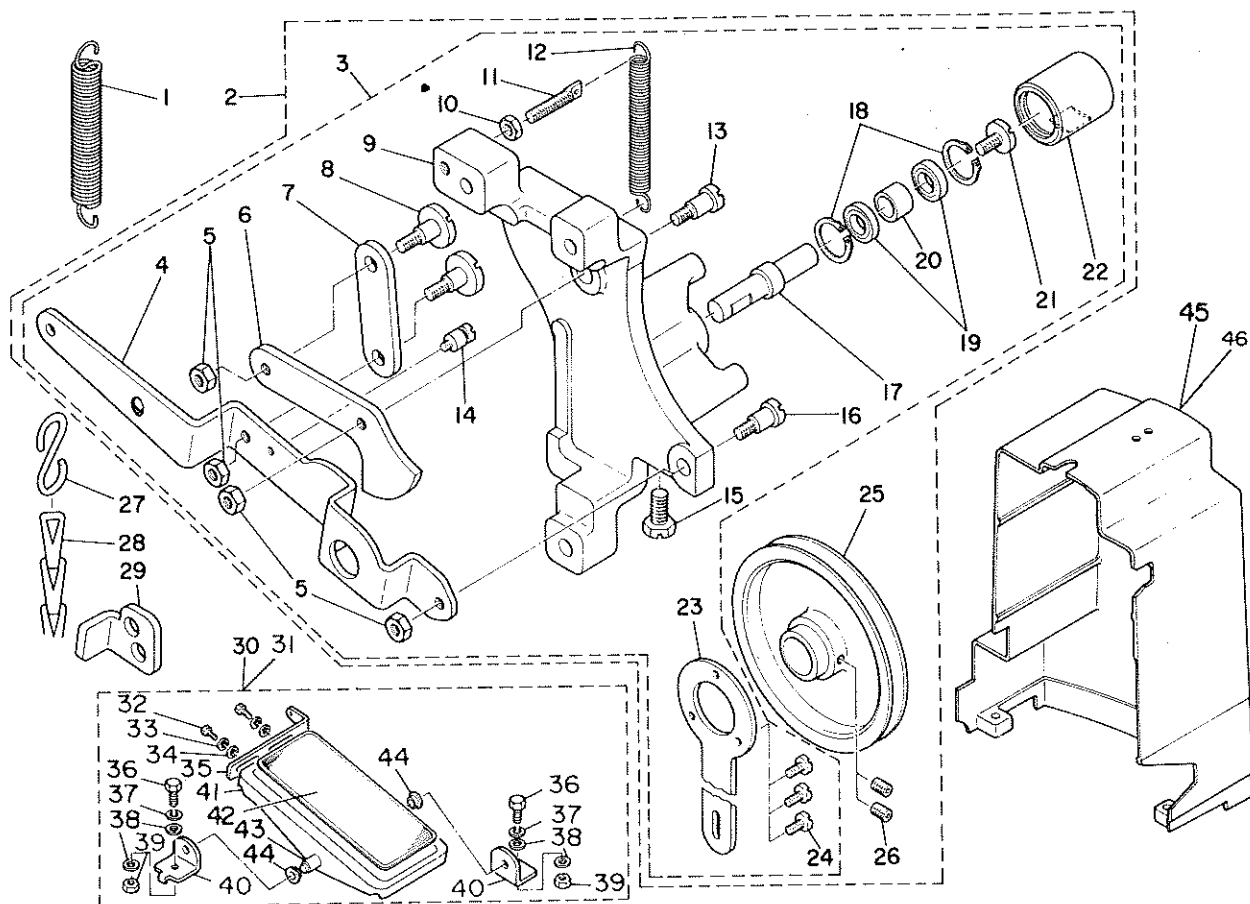
(14) LK-1850-P PEDAL TYPE CLAMP FOOT LIFTING DEVICE 足踏式押上げ装置
