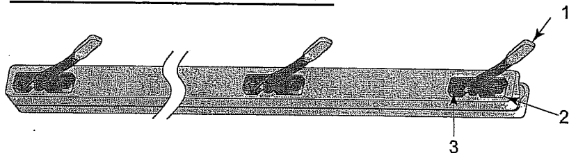
BSC-B000 One-touch Special Clip
