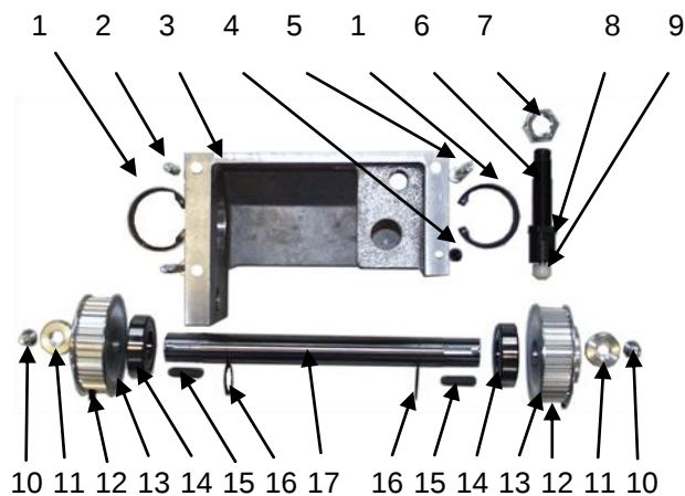
Return pulley compl. Item: 115411
