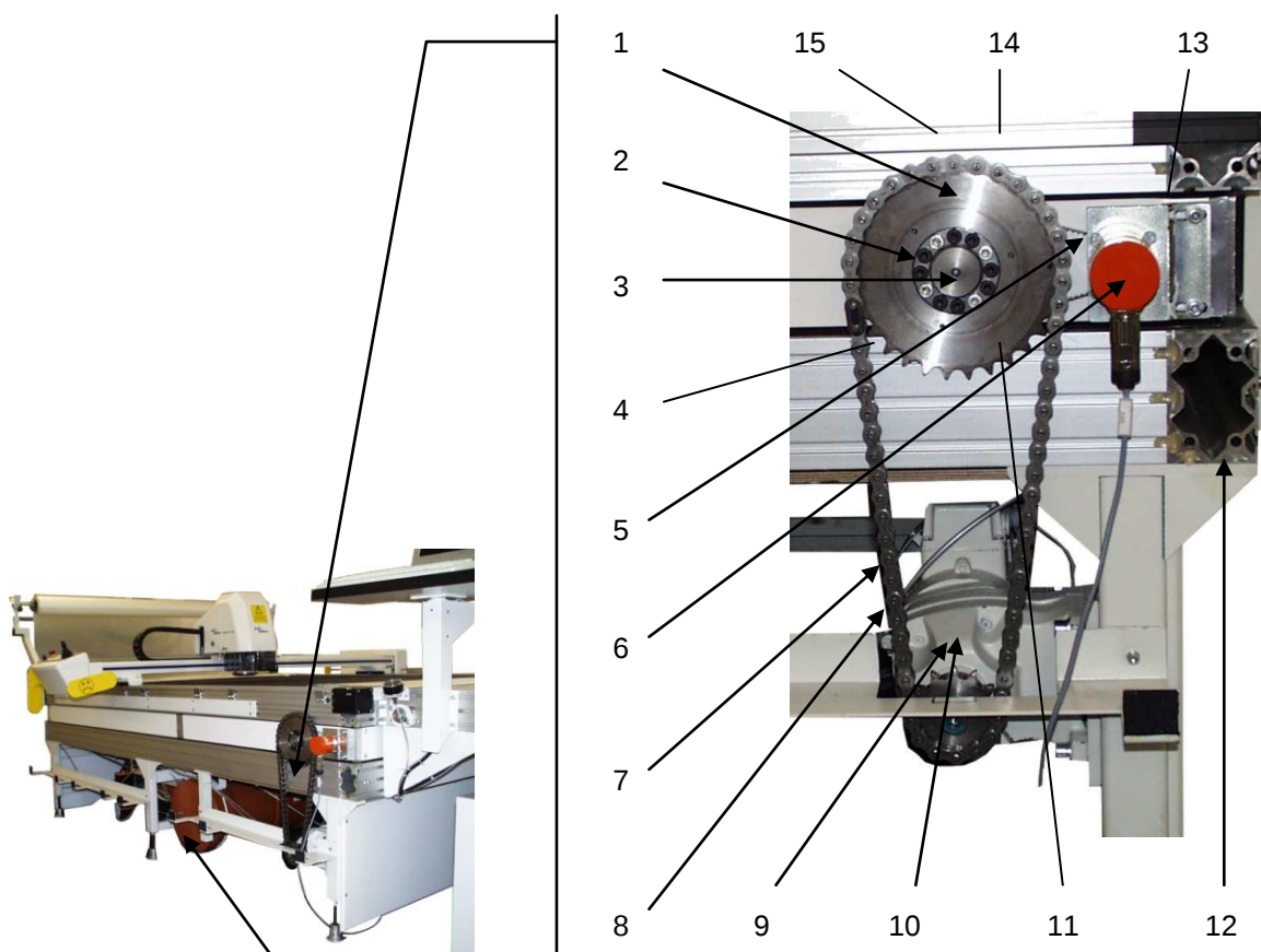
>Conveyor Drive<
