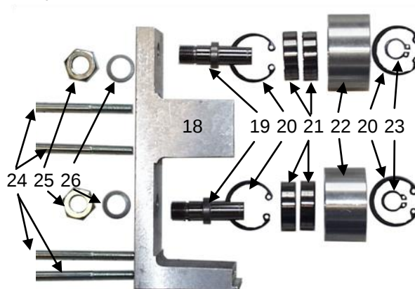
Return pulley compl. Item: 115411
