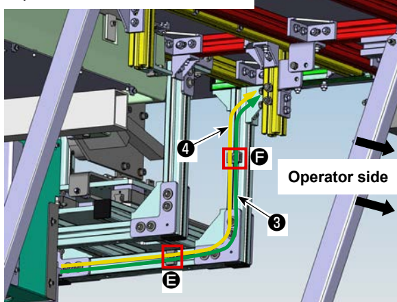
3) BK left side rear view
