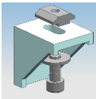
⑩ Two sets of small angle brackets (Small angle bracket x 1 piece, M6×14 screw x 2 pieces, M6 slide nut x 2 pieces, plain washer of outside diameter \varnothing 17 x 2 pieces)
