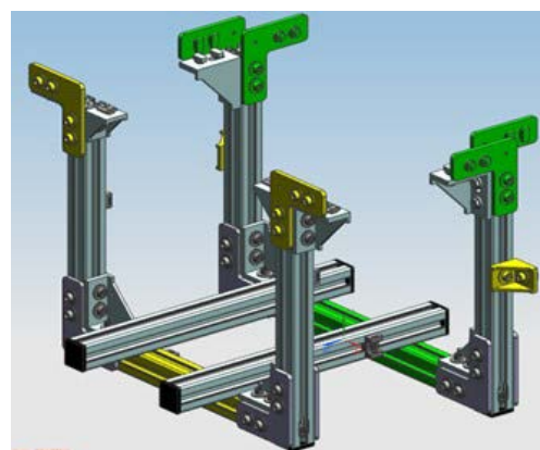
PS-910-6055 Reference drawing of the completed state of the aluminum frames
