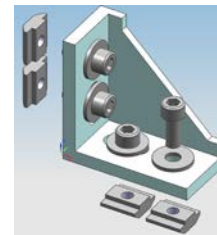
⑧ Two sets of large angle brackets (A) (Large angle bracket x 1 piece, M6 x 14 screw x 4 pieces, M6 slide nut x 4 pieces, plain washer of outside diameter ø17 x 4 pieces)
