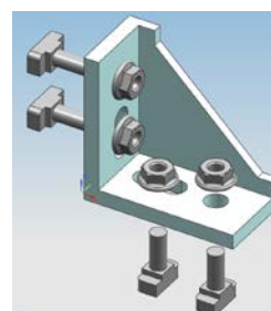
⑪ Two sets of large angle brackets (Large angle bracket x 1 piece; M6 flange nut x 4 pieces; M6 aluminum frame dedicated screw x 4 pieces)
