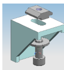
⑫ Two sets of small angle brackets (Small angle bracket x 1 piece, M6 x 14 screw x 2 pieces, M6 slide nut x 2 pieces, plain washer of outside diameter Ø17 x 2 pieces)
