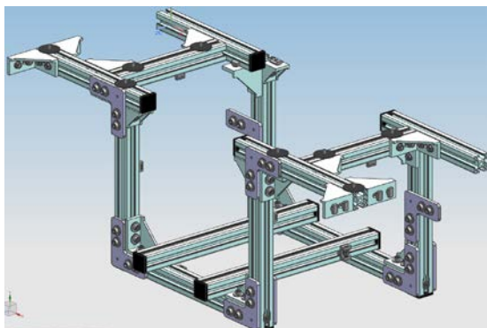
PS-900/PS-910-13090 Reference drawing of the completed state of the aluminum frames
