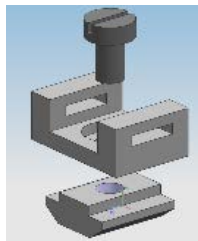
Three sets of cable fixtures (Fixing base + M6 flange nut + Slotted head screw M5 x 8L)
