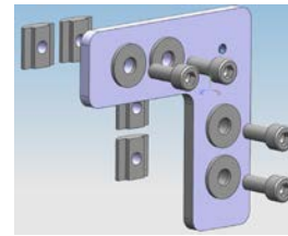
⑦ Six sets of link plates (A) (Link plate x 1 piece, M6 x 14 screw x 4 pieces, M6 slide nut x 4 pieces, plain washer of outside diameter ø17 x 4 pieces)
