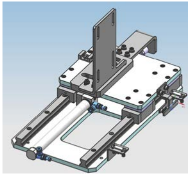
One set of the lengthwise feed base
