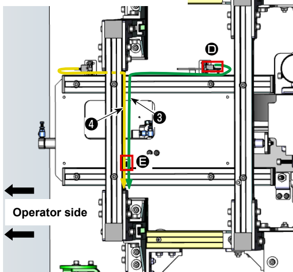
2)-2. Bottom view of the table
